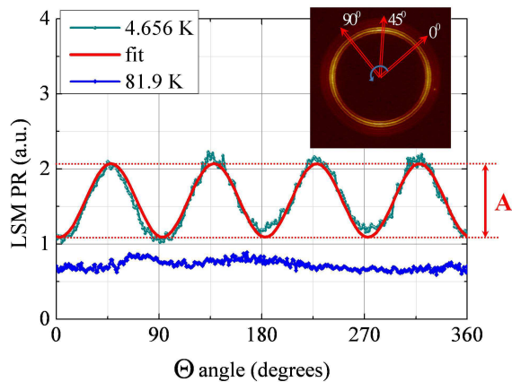
FIG. 2. Plot of radially-integrated and unwrapped photoresponse (PR) vs. angle on the YBCO/LAO spiral at 81.9 K and 4.66 K, along with a fit of the low-temperature integrated PR( \Theta ) to the simple d-wave angular dependence. Inset shows PR image of YBCO/LaAlO 3 thin film spiral resonator taken at a temperature of 4.656 K in the 7 th mode at 450.22 MHz.
