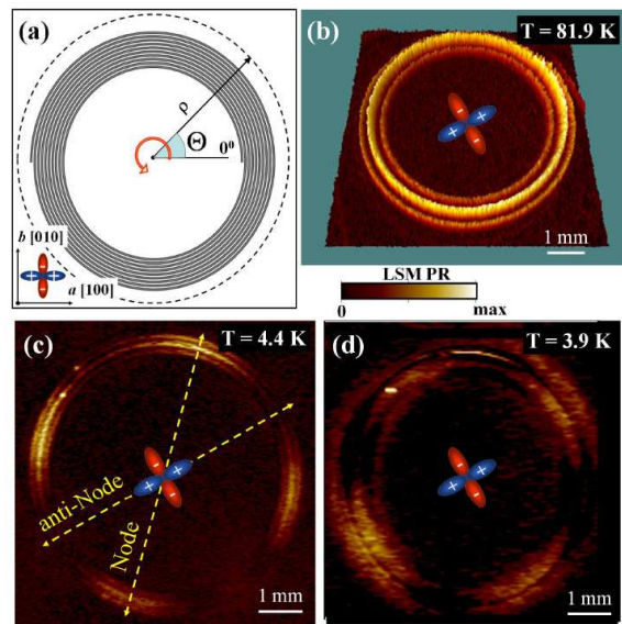
FIG. 1. a) Schematic diagram of spiral geometry, definition of radial ( \rho ) and angular ( \Theta ) coordinates, and directions of the crystallographic a- and b-directions, along with the orientation of the d-wave gap in YBCO. b)-d) LSM photoresponse images of a YBCO/LAO spiral resonator in the third harmonic mode at temperatures of b) 81.9 K, c) 4.40 K, d) 3.90 K. Also shown is the d-wave gap orientation as determined from twin domain boundary directions in the substrate.
