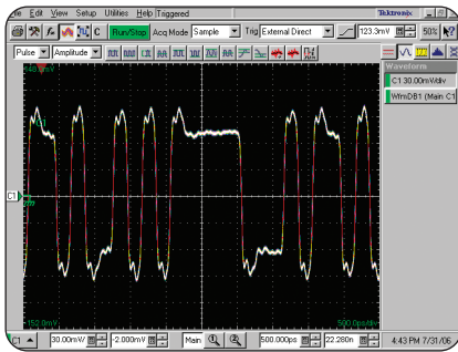
► Figure 1: 5 Gb/s Pre/De-emphasized signal.
