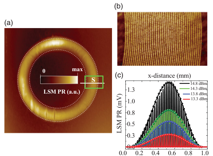
FIG. 3. (Color online) (a) 2D LSM image showing current distributions in a Nb spiral with an outer diameter of 6 mm and 40 turns, at the fundamental resonant mode of 74 MHz, T_B = 4.5 \text{ K} , P_{\text{rf}} = 14.8 \text{ dBm} . (b) 2D LSM reflectivity image showing the individual turns within an area on the spiral marked with a green box in (a). (c) The power-dependent \text{PR}_R along the cross section of the spiral shown with S line; maximum at the center, minimum at the edges. The dots are the estimated J_{\text{rf}}^2 profile for a simple standing wave current pattern at each P_{\text{rf}} .
