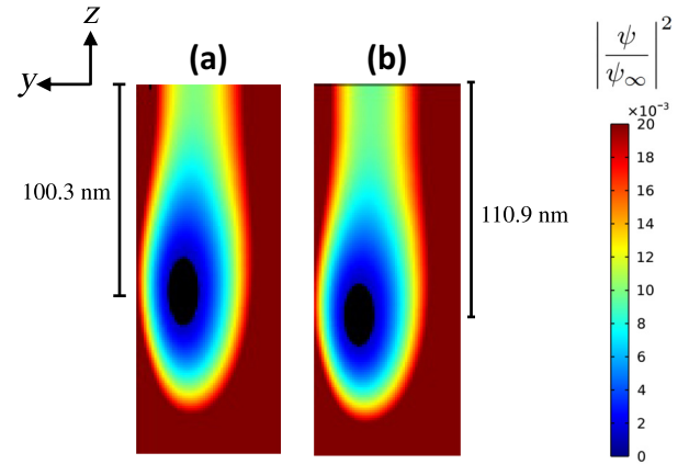
FIG. 20. A snapshot of the vortex core obtained by the TDGL simulation for the grain-boundary model in Sec. IV C for B_{pk} = 50.9 mT (a) and for B_{pk} = 56.6 mT (b), with the temperature being 5.5 K and h_{penetration}^{defect} = 200 nm. This snapshot is taken when the rf field reaches its maximum in an rf cycle [ \omega t = \pi/2 and hence B_{rf} \sin(\omega t) = B_{rf} ]. The snapshot shows the distribution of the square of the normalized order parameter on the Y - Z plane immediately below the dipole around the grain boundary that nucleates an rf vortex semiloop. The black region is where |\psi/\psi_\infty|^2 < 0.001 .
