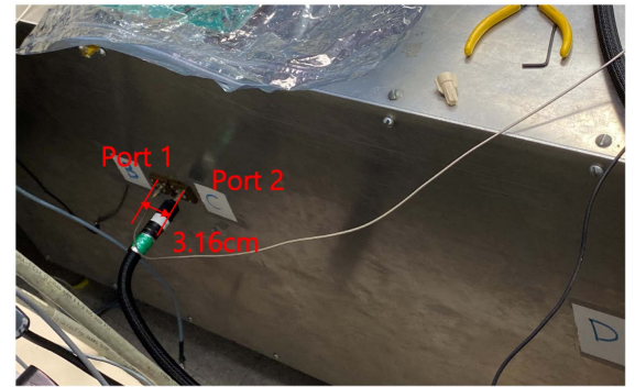
Fig. 13. Measurement configuration of nearby antennas.
