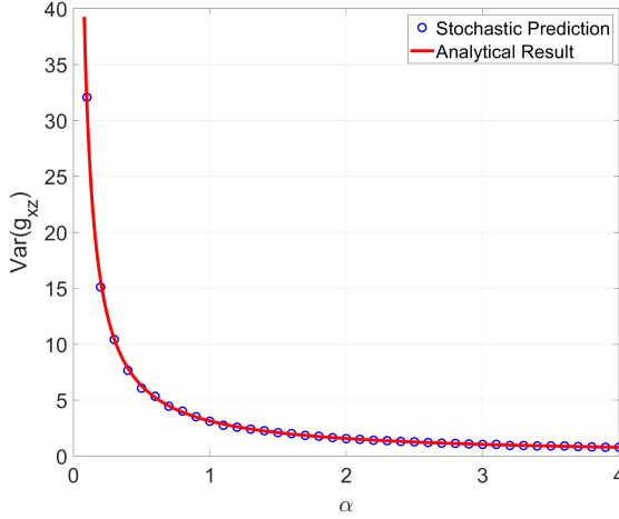
Fig. 17. Variance of g_{xz} with increasing \alpha .
