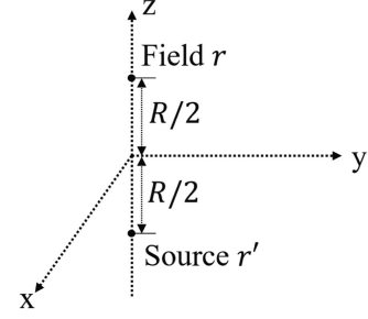
Fig. 1. Notation for the covariance derivation.
