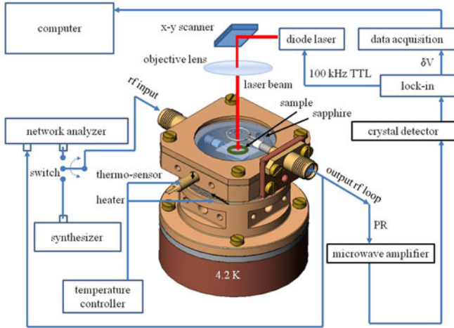
Fig. 4. Schematic of the laser microscope test setup arrangement. A spiral resonator is mounted in the cryostat between the two magnetic loop probes. The probing signal is injected through the upper loop and received at the lower magnetic probe. The sample is scanned with a focused laser beam, generating locally the quasi-particles and inducing the loss. The induced loss is also proportional to the local amplitude of RF current. When mapping the laser beam induced losses over the sample (with RF signal applied), we obtain the map of RF currents in the sample [12].
