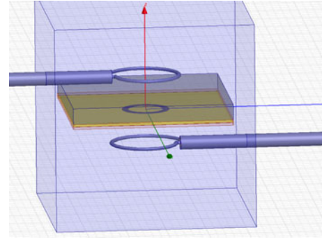
Fig. 2. Experimental RF test setup as simulated numerically in HFSS. A sample of twin-spiral resonator is placed between the two RF loop probes. The two loops probes are weakly magnetically coupled with each other and with the ring shaped resonator. At the resonance frequencies of the two-spiral structure the loop coupling ( S_{21} ) increases substantially (see Fig. 3 and 5).
