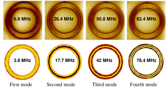
Fig. 5. RF current distribution measured with LSM (above) and HFSS simulated (below) for the first 4 inner modes of the two-spiral resonator. The brighter color corresponds to the higher RF current density. The number of antinodes is equal to the mode number. The capacitive overlap areas do not have pronounced nodal structure in experimental data. The bright background in experimental data is due to a strong photo response in the Si substrate of the tested sample. The measured and calculated resonance frequencies are listed in the middle of each plot.
