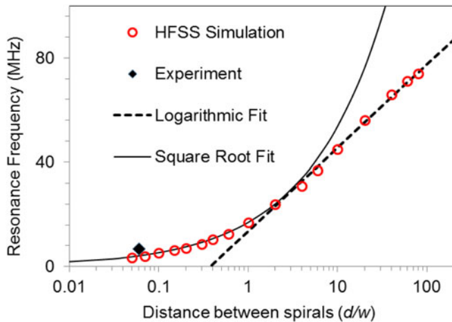
Fig. 6. Twin-spiral resonator fundamental resonance frequency as a function of the ratio of distance ( d ) between the two spirals to the width of the spiral line ( w ) simulated with HFSS (open circles). All other twin-spiral dimensions are the same, as presented in Fig. 3. For the spacing larger than 15 \mu\text{m} ( d/w = 3 ) the resonance frequency dependence versus d is logarithmic, and below the 10 \mu\text{m} distance ( d/w = 2 ) the resonance frequency goes as a square root of the distance. The measured resonance frequency of 6.9 MHz (see Fig. 3) fits reasonably well the HFSS simulated data for the distance d of 300 nm, typical for the thickness of dielectric layer in the tested sample. One can note the 12 fold reduction of the fundamental resonance frequency in the two spiral resonator compared to the single spiral resonance frequency of about 83 MHz.
