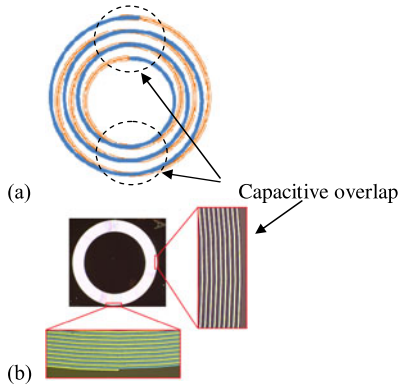
Fig. 1. (a) A sketch of the two-spiral resonator. The two planar Archimedean spirals are superposed with a thin dielectric layer in between. Spirals are identical in shape and turning in opposite directions: one clockwise, another counter-clockwise. Both spirals are shaped as a ring, with no central part. The spiral arms overlaps play a role of interlayer capacitors, when the other sections of the spiral are still highly inductive, as in a free standing spiral. The additional capacitive loading leads to the reduction of speed of propagation of the signals along the spirals. The spirals act as a distributed RF resonator with multiple modes, and the reduction of the phase speed in the structure gives a lower resonance frequency. The two-spiral structure is made by photo lithography as a three layer circuit. (b) A photo of the two-spiral resonator used in our experiment. At the left blow-up image the windings of the two spirals are matched (overlapped), forming capacitive elements, at the bottom blow-up image the windings are mismatched because the two spirals are turning in the opposite directions.
