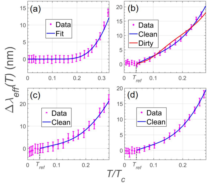
FIG. 3. \Delta\lambda_{\text{eff}}(T) vs T/T_c data and fits for SmB 6 /YB 6 bilayers at low temperature, T/T_c < 0.3 . (a) The single-layer YB 6 (100 nm) ( t_{\text{SmB}_6} = 0 nm). The magenta points are data, and the blue line is a fit from the electromagnetic screening model. (b) The bilayer with t_{\text{SmB}_6} = 20 nm. The blue line is a fit with the clean-limit temperature dependence of \xi_N(T) , and the red line is a fit with the dirty-limit temperature dependence. [(c) and (d)] The bilayers with t_{\text{SmB}_6} = 40 nm and 100 nm, respectively.
