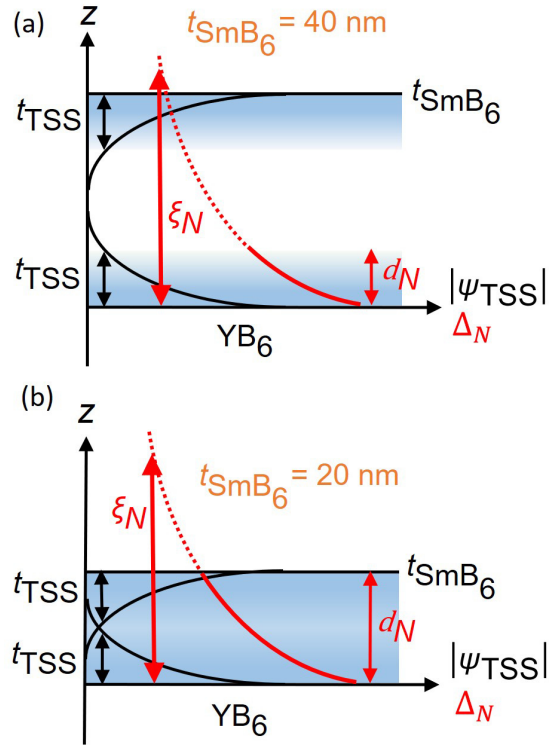
FIG. 4. Schematic view (not to scale) of the proposed position dependence of the surface states wave function |\psi_{\text{TSS}}(z)| (black) and induced order parameter \Delta_N(z) (red) in the \text{SmB}_6/\text{YB}_6 bilayer for the case of t_{\text{SmB}_6} = (a) 40 nm, and (b) 20 nm. The |\psi_{\text{TSS}}(z)| is also visualized by the blue gradations in the \text{SmB}_6 layer. The sketches are based on the estimated normal coherence length \xi_N(2\text{K}) = 52 nm and the surface state thickness t_{\text{TSS}} \approx 9 nm. In a thick \text{SmB}_6 layer (a), only the bottom surface is proximitized so that d_N = t_{\text{TSS}} = 9 nm. In a thin \text{SmB}_6 layer (b), through the wave function overlap between the top and bottom surface states, the entire \text{SmB}_6 layer is proximitized so that d_N = t_{\text{SmB}_6} = 20 nm.
