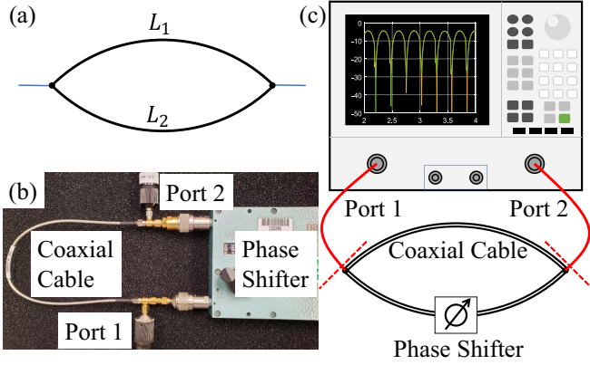
FIG. 1. (a) Schematic diagram of a generic ring graph connected to two infinite leads. The two bonds have length L_1 and L_2 . (b) Picture of the experimental microwave ring graph, where a coaxial cable and a coaxial microwave phase shifter are used as the two bonds. (c) Schematic of the experimental setup with the microwave network analyzer included. The two dashed red lines indicate the calibration plane for the 2 \times 2 S-matrix measurement.
